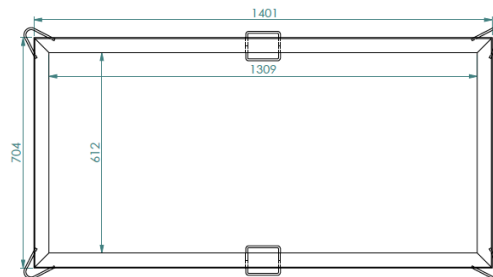
Concrete Infill cross-section top view
