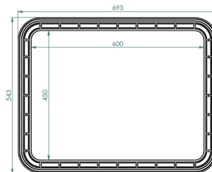
Modula cross-section top view
